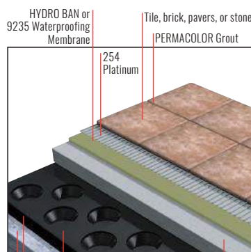
Tile Drain Mat Primary roof waterproofing membrane Structural concrete deck, properly pitched
